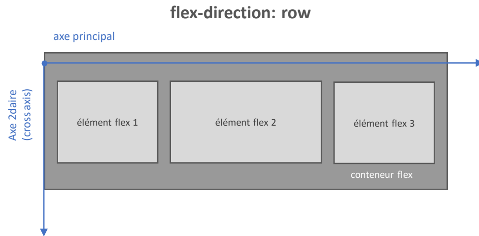
Figure 44: Exemple de flex-direction row
